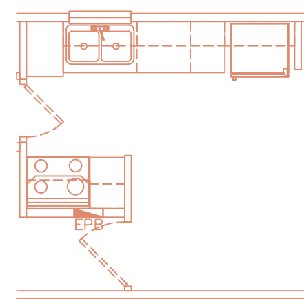
OPT. DISHWASHER CONFIGURATION
