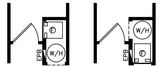
FLOOR DUCT OVERHEAD DUCT FURNACE / AIR HANDLER OPTION
